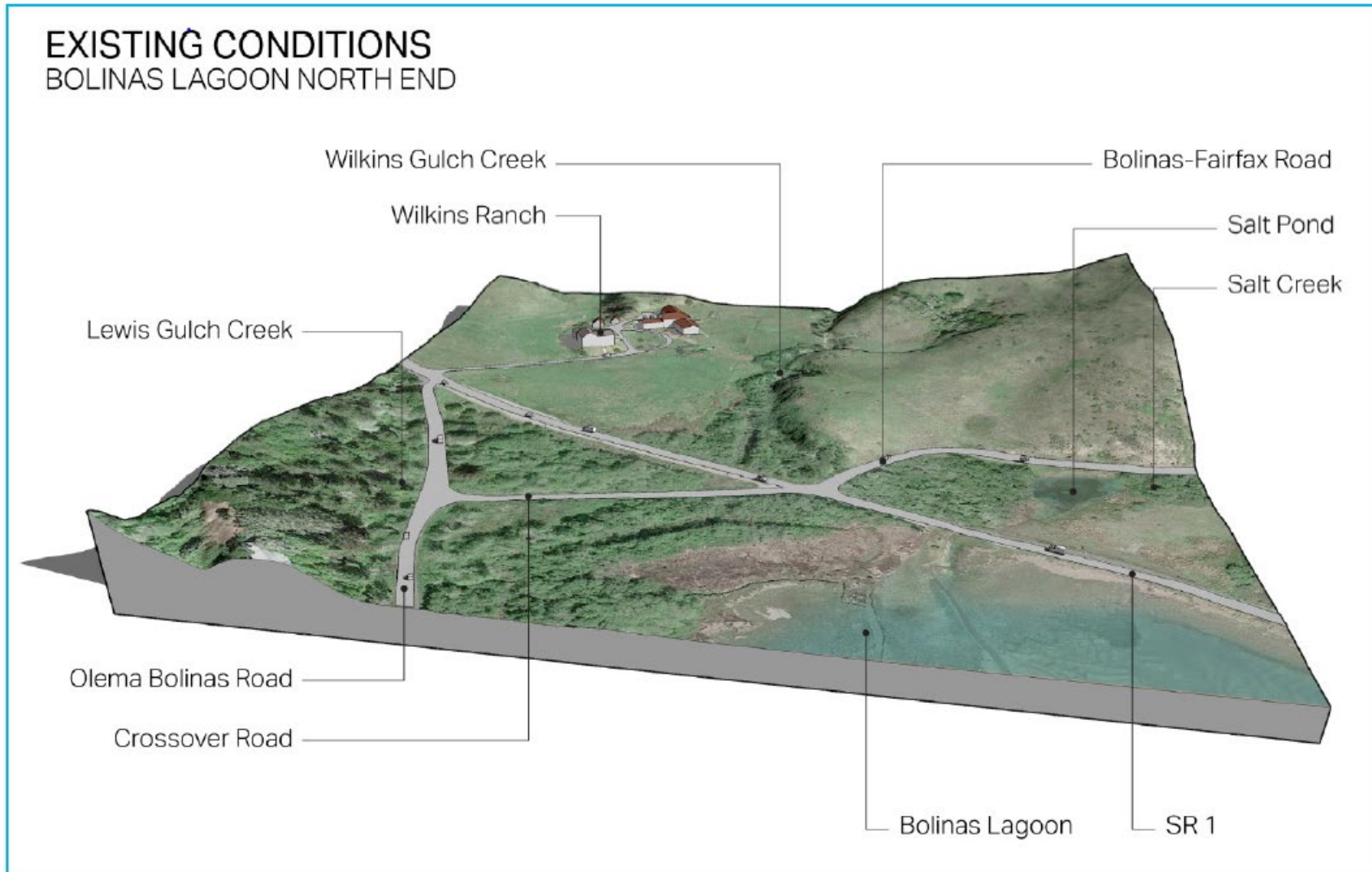
Figure 2: Existing Conditions - North End of Bolinas Lagoon
