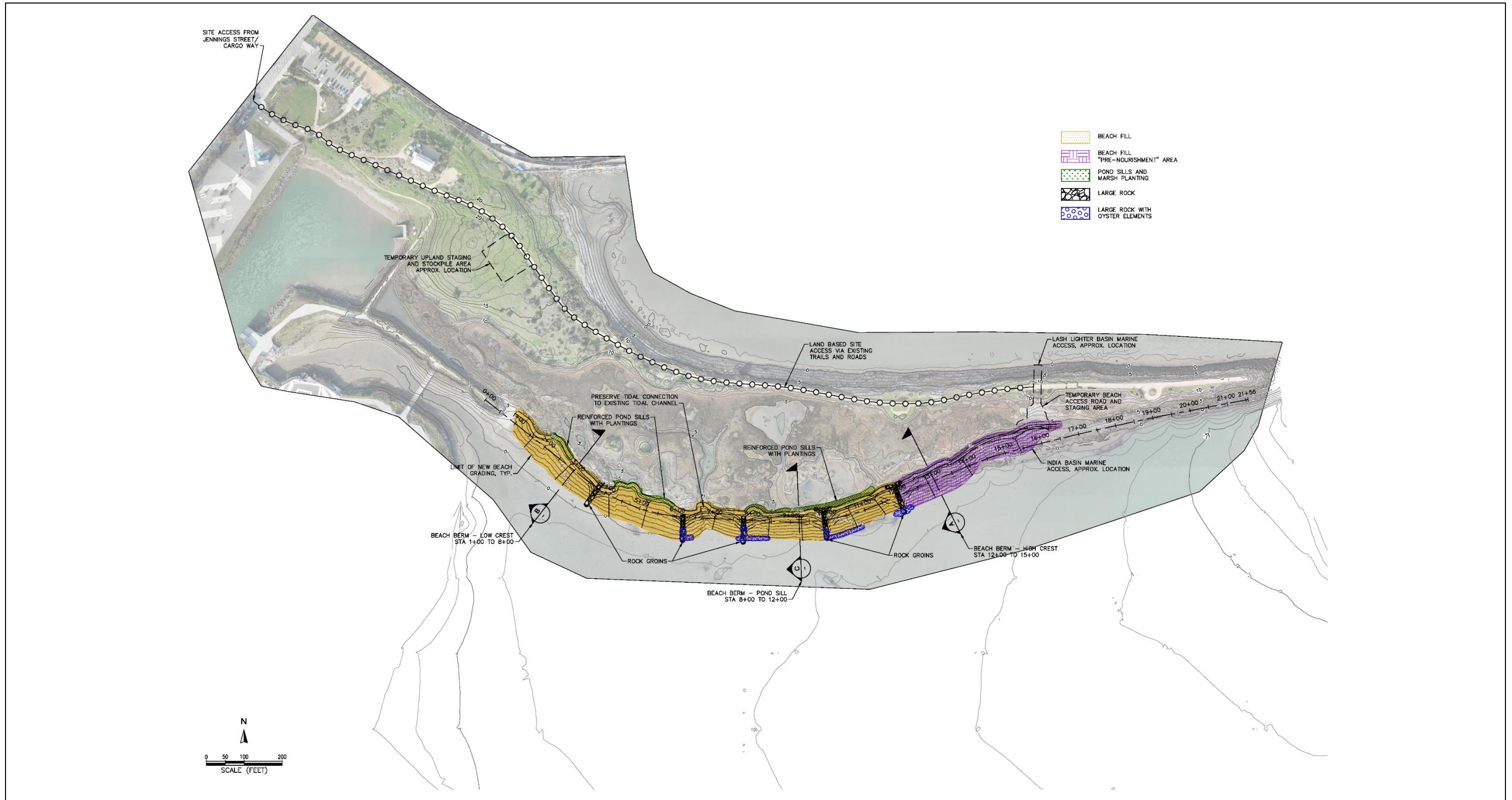
Heron's Head Shoreline Resiliency Project Figure A-3 Proposed Project
